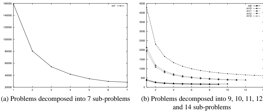
Fig. 5. Execution time in logistics problems when using up to 14 processors (x axis represents the number of processors used and y axis indicates time in ms.)
