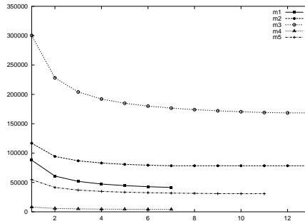
Fig. 6. Execution time in depots problems when using up to 13 processors.
